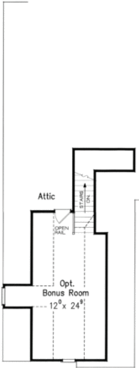
OPT. BONUS ROOM PLAN
